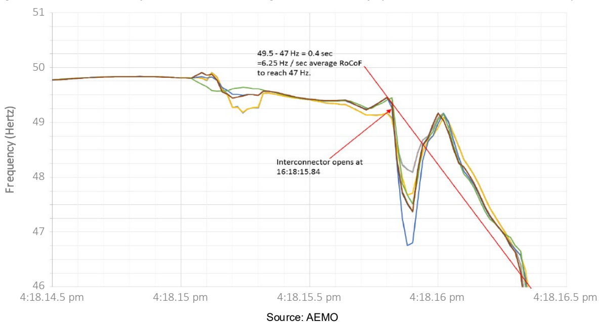
Figure 11 - Frequency and Rate of Change of Frequency (various measurement points)
