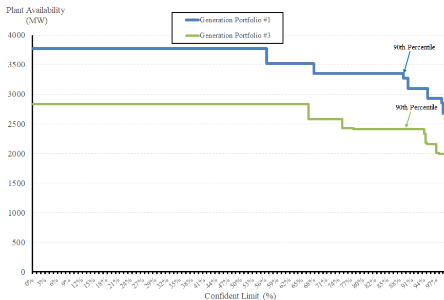
Figure 4: Primary supply of hedge contracts at 0% VRE Market Share
