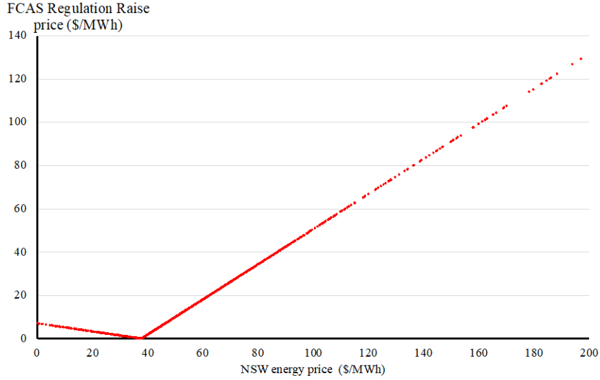
Figure 8: Theoretical model of FCAS Regulation Prices in the NSW region
