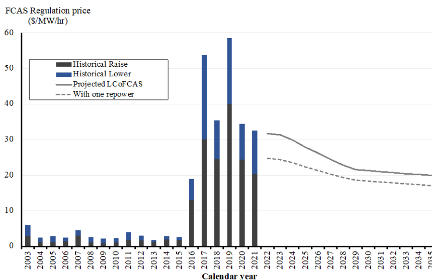
Figure 13: Projected LCoFCAS Regulation from grid-scale batteries
