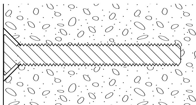
GU001 REMOVABLE MOUNTING METHOD "REMOVED" SCALE 1:1
