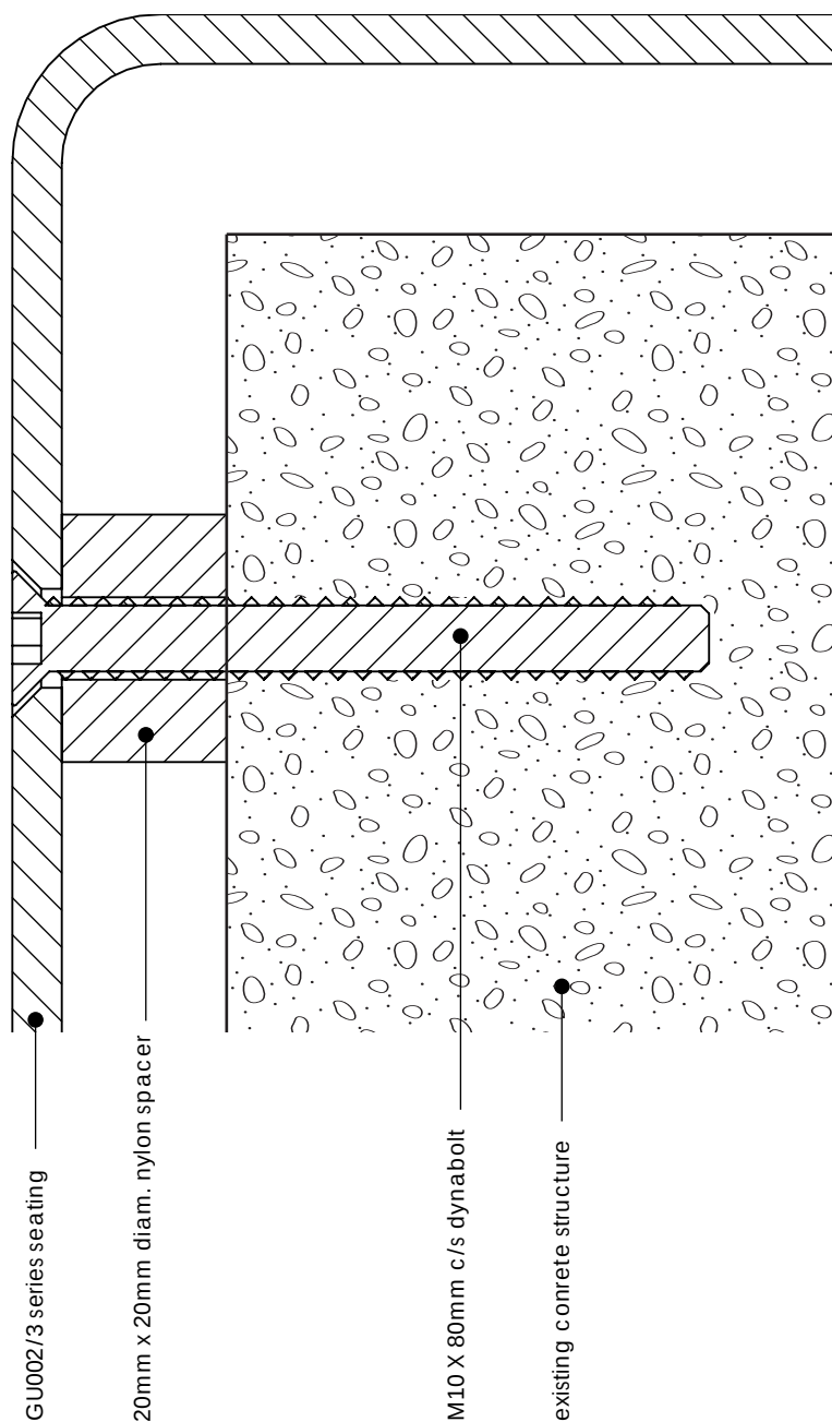
GU002/GU003 MOUNTING METHOD SCALE 1:1
