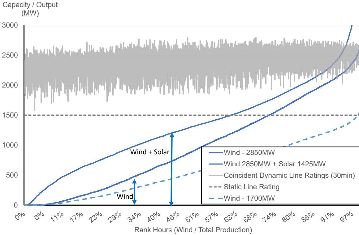
Figure 8 - Wind Output and VRE portfolio output (ranked) vs Dynamic Line Ratings 12
