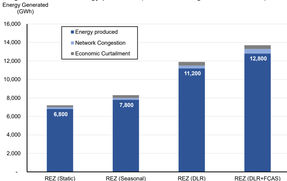
Figure 10 - VRE energy produced (fleet-wide congestion \geq 1% ACF)
