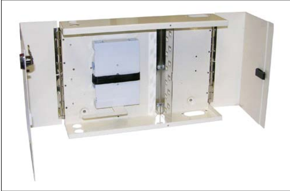
Figure 19 Optic Fibre Splice Tray and Patch Panel
