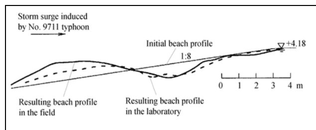
Figure 1. Validation of the moveable bed model through comparison of the beach profile created in the laboratory and that resulting from the storm surge induced by typhoon No 9711
