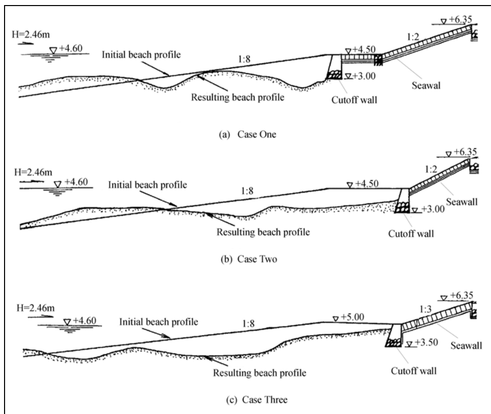
Figure 2. Resulting profile configurations with different kinds of seawalls under erosive wave conditions with a 50-year return period. An initial profile with a face slope of 1:8 was determined by the situation of artificial sandy beaches on the coast of Northern Jiangsu Province, China. Each test was run for a 24 hours prototype wave action.
