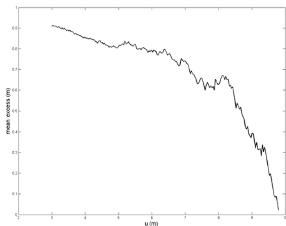
Figure 2. Mean excess plot for different thresholds values.
