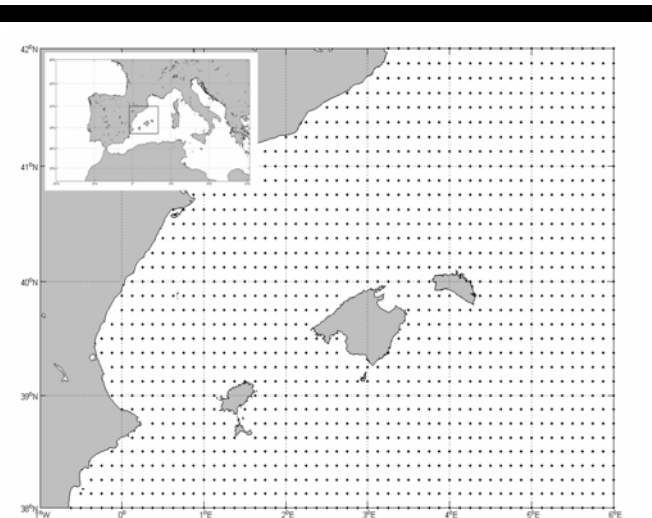
Figure 1. Geographic location of the study area and the 1/8^\circ resolution HIPOCAS grid over the Balearic Sea.
