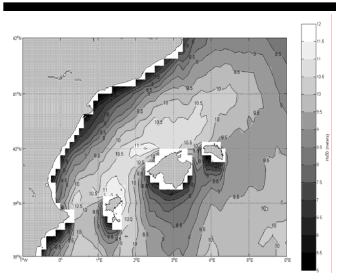
Figure 5. Spatial distribution of H_{s50}
